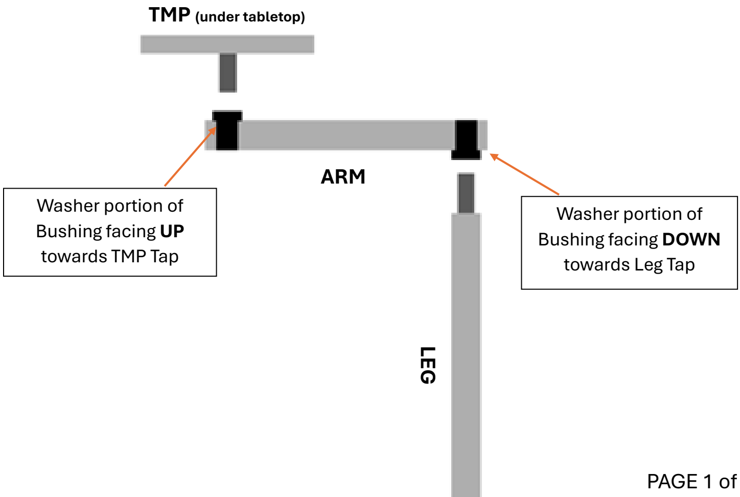
Washer portion of Bushing faces towards Taps
